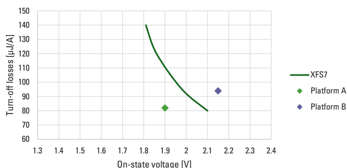
1200 V Technology Platform Comparison
