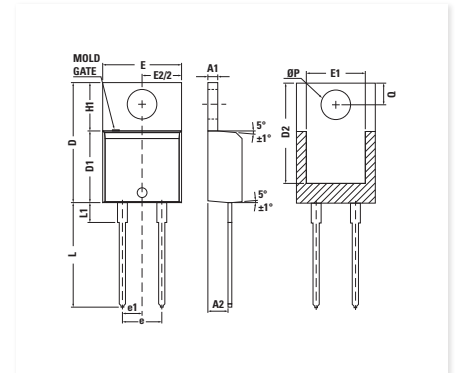
L005b TO-220AC Weight = 2 g
