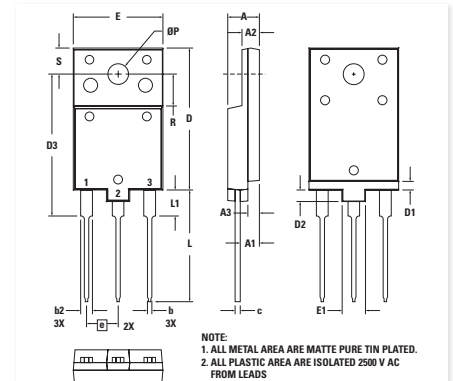
X017c TO-3PFP Weight = 5.5 g
