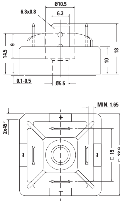
X122 PWS-D
