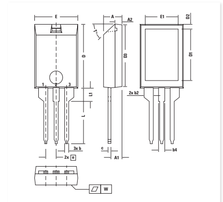
X010a ISOPLUS220™ AB Weight = 2.5 g
