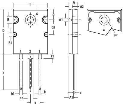
X020a TO-264 AA Weight = 10 g
