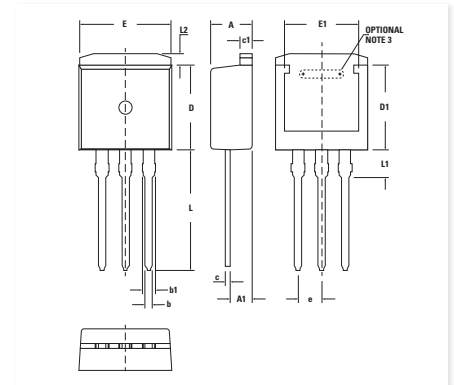
X008a TO-262 I2PAK Weight = 1.5 g
