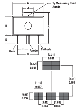
L016 SOT-89 Weight = 0.045 g
