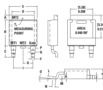
L004 TO-252AA Weight = 0.3 g
