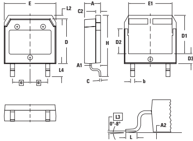
X019a TO-268 AA (D3PAK HV) Weight = 4 g
