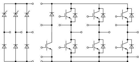
6-Pack
