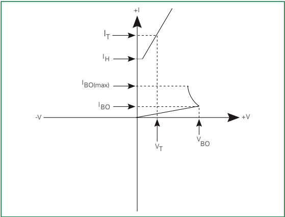
Figure 1. Typical V-I Characteristics
