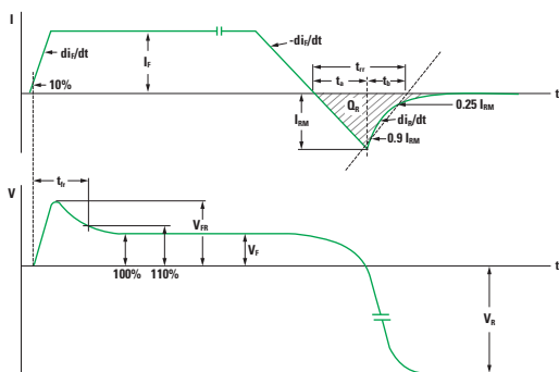
Current and Voltage During Turn-On and Turn-Off Switching of Fast Diodes
