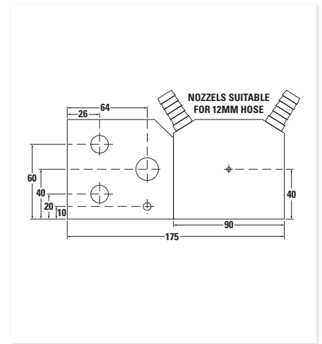
WCL3 - LKB COOLER
