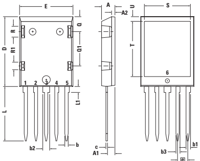
X022 ISOPLUS264™ Weight = 7.5 g
