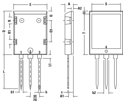
X022a ISOPLUS264™ Weight = 7.5 g
