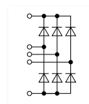
3-phase, B6U
