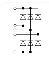
Three-Phase, B6U
