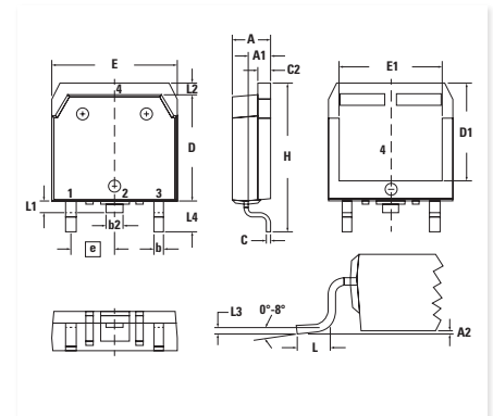
X019 TO-268 AA (D3PAK) Weight = 4 g
