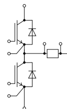
Phase Leg + Shunt
