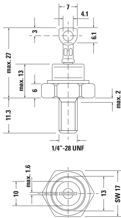
X207 DO-203 AB (DO-5) Weight = 20 g
