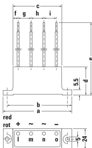
X252 UG Weight = 155 g
